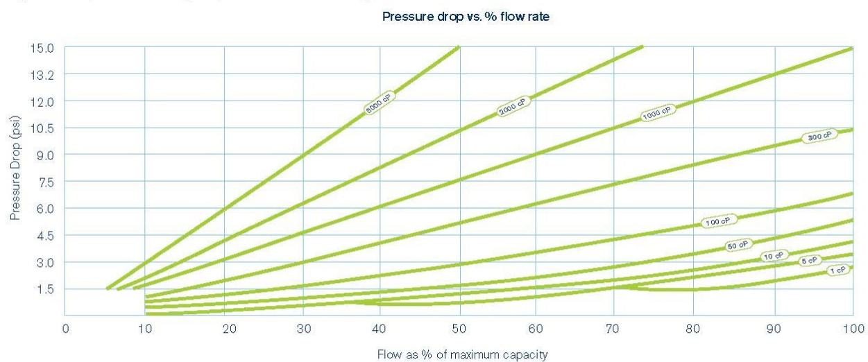
Figure 7: Impact of viscosity on pressure loss for a range of flow rates
